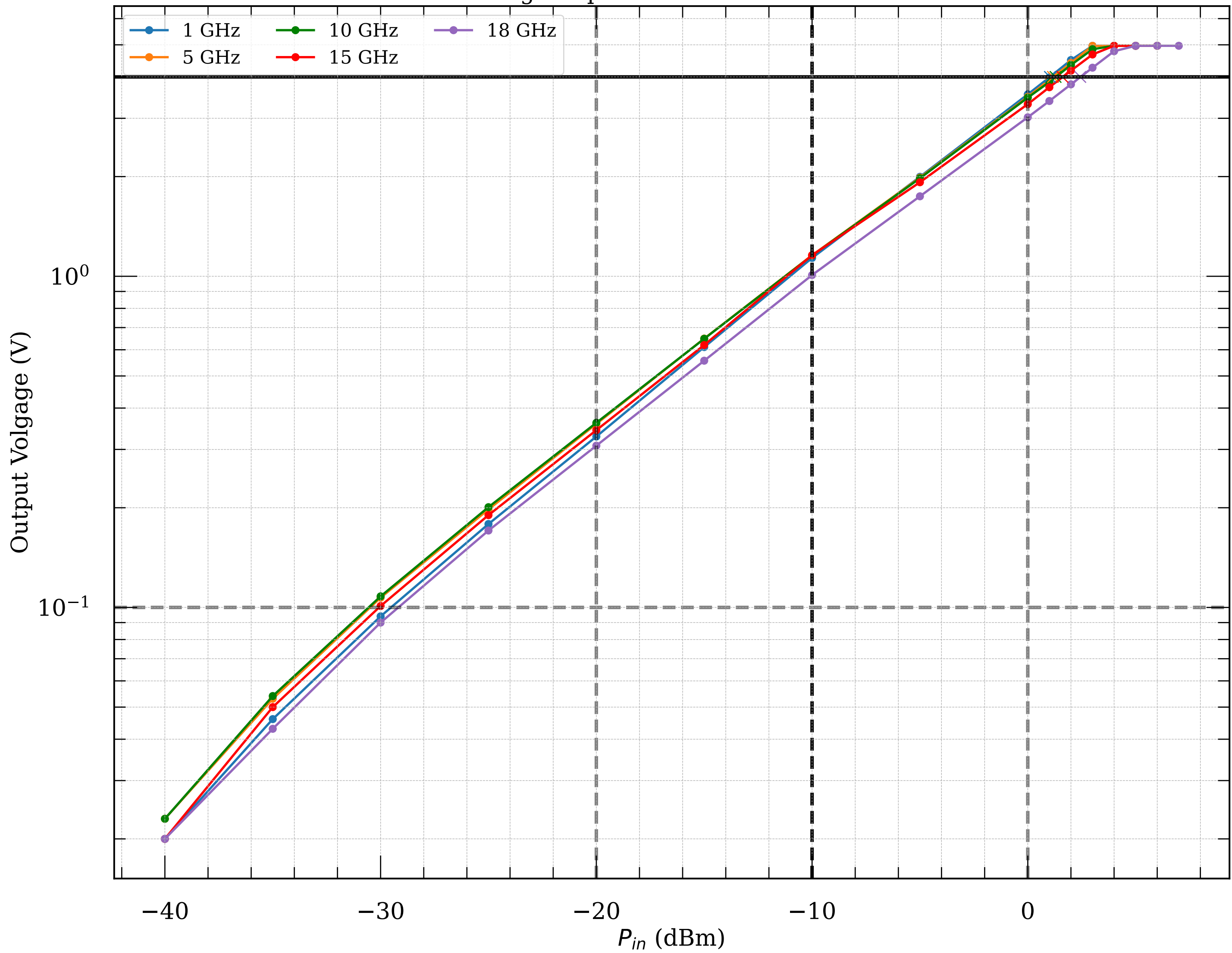
Measured voltage-to-power curve of detector module099
